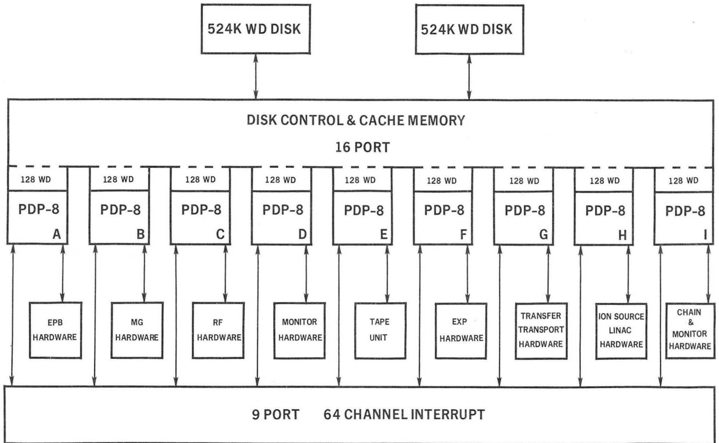
Fig. 3 - Existing System Block Diagram
