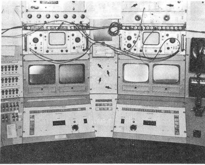
Fig. 5 - External Proton Beam Control Station
