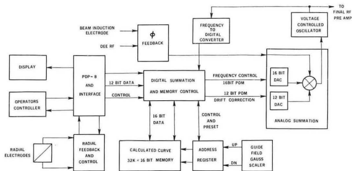
Fig. 9 - RF System Block System
