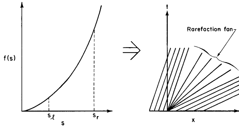
Fig. 1—Riemann problem solution, convex f(s) , s_l < s_r .
