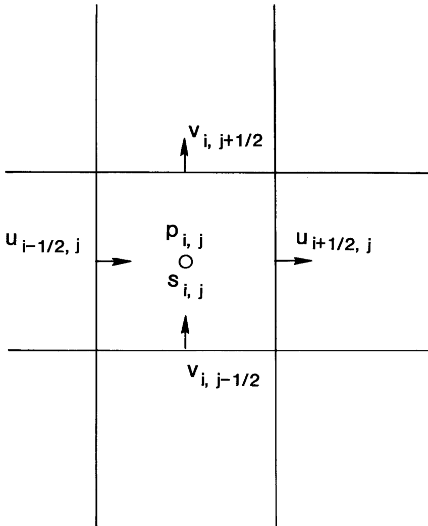
Fig. 6—Staggered grid for p , s , and \bar{u} .
