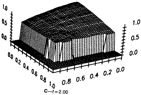
Fig. 8—Saturation for 40×40 diagonal grid.
