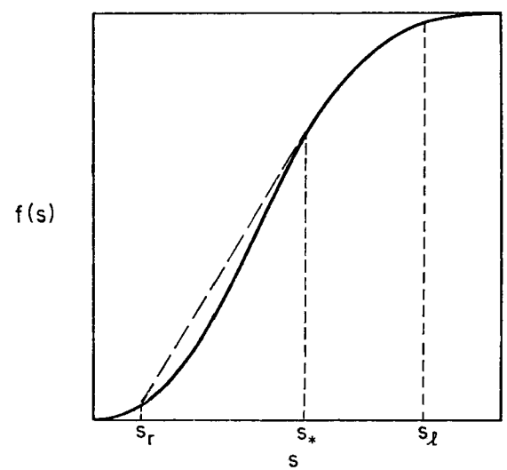
Fig. 4—Convex hull for compound wave solution, s_l > s_r .
