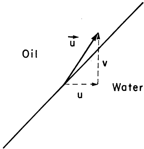
Fig. 5—Obliquely propagating discontinuity front.
