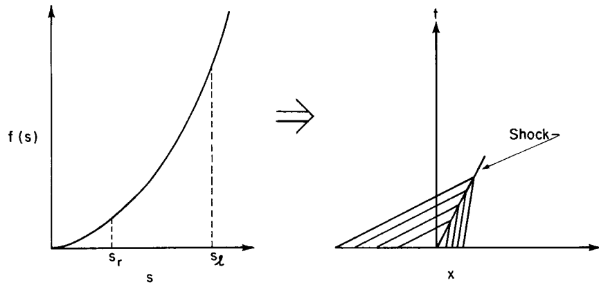
Fig. 2—Riemann problem solution, convex f(s) , s_l > s_r .
