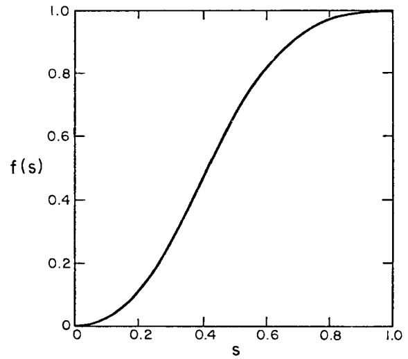
Fig. 3—Fractional flow function.
