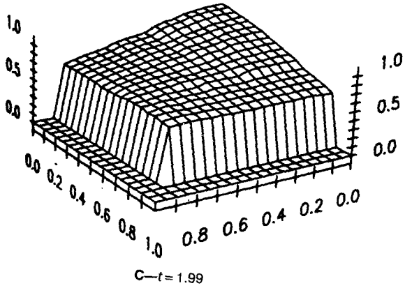
Fig. 7—Saturation for 20×20 diagonal grid.
